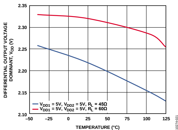
Figure 14. Driver Differential Output Voltage Dominant vs. Temperature
