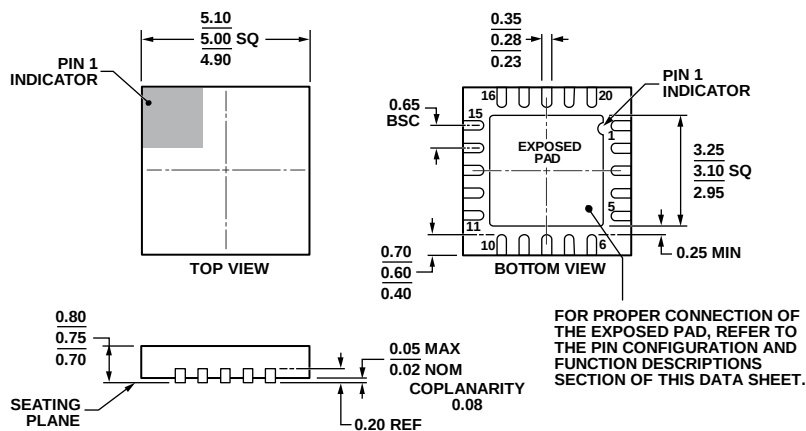
COMPLIANT TO JEDEC STANDARDS MO-220-WHHC. Figure 68. 20-Lead Lead Frame Chip Scale Package [LFCSP_WQ] 5 mm x 5 mm Body, Very Very Thin Quad (CP-20-9) Dimensions shown in millimeters
