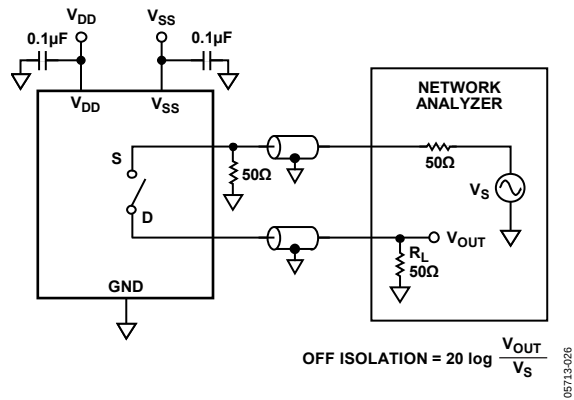
Figure 38. Off Isolation
