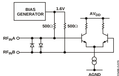
Figure 29. RF Input Stage
