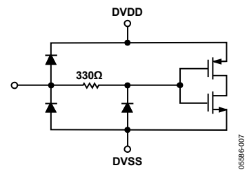
Figure 11. Digital Inputs
