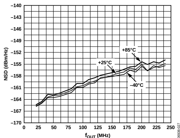
Figure 27. AD9783 One-Tone NSD vs. f_{OUT} Over Temperature, at 500 MSPS, FS = 20\text{ mA}
