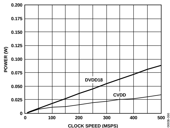
Figure 69. Power Dissipation, Digital 1.8 V Supply, Clock 1.8 V Supply, I Data Only
