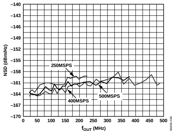
Figure 26. AD9783 Eight-Tone NSD vs. f_{OUT} Over f_{DAC} Baseband and Mix Modes, FS = 20\text{ mA}
