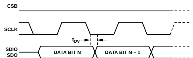
Figure 55. Timing Diagram for SPI Read Register
