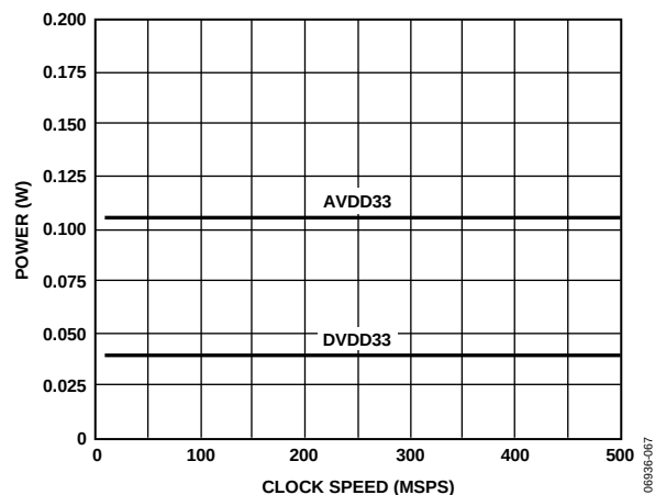
Figure 70. Power Dissipation, Digital 3.3 V Supply, Analog 3.3 V Supply, I Data Only
