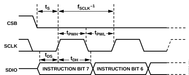
Figure 54. Timing Diagram for SPI Write Register
