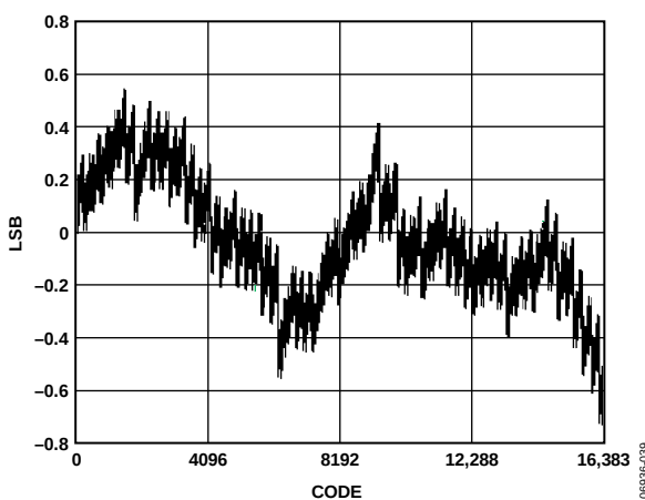
Figure 39. AD9781 INL, FS = 20 mA
