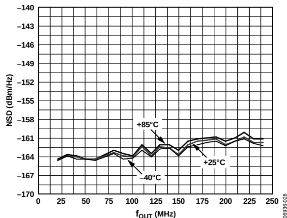
Figure 28. AD9783 Eight-Tone NSD vs. f_{OUT} Over Temperature, at 500 MSPS, FS = 20\text{ mA}
