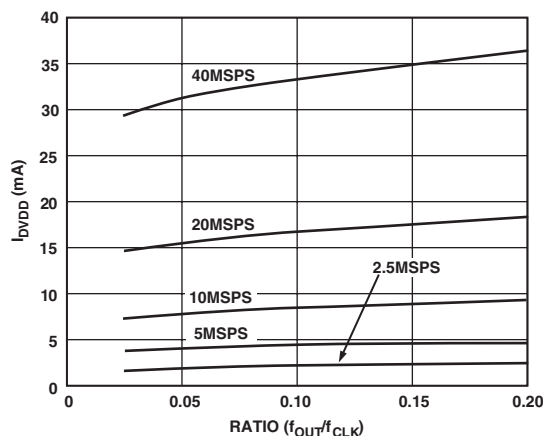
Figure 16. I_{DVDD} vs. Ratio @ DVDD = 3V
