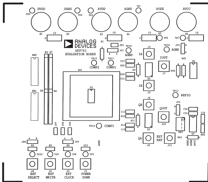
Figure 25. Silkscreen Layer—Top
