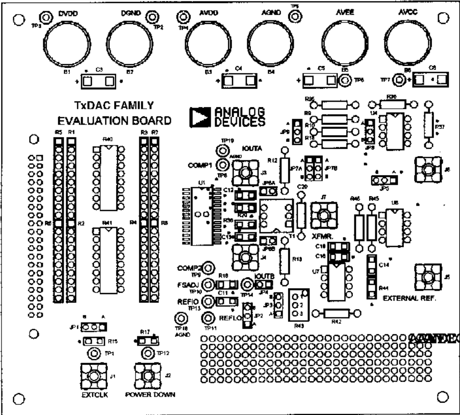
Figure 27. Silkscreen Layer—Top
