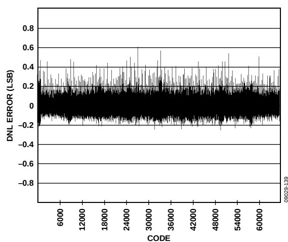
Figure 39. DNL, f_{IN} = 4.3 MHz, 2.5 V p-p FS, AD9467-250
