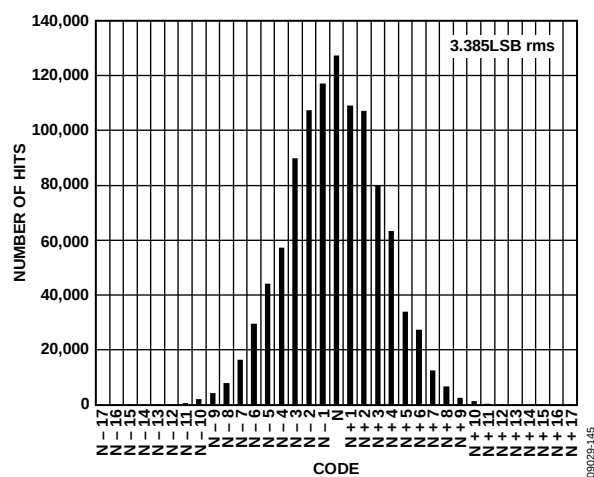
Figure 45. Input-Referred Noise Histogram, 2.5 \text{ V p-p FS} , AD9467-250
