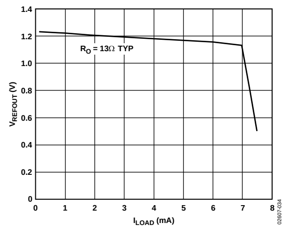
Figure 34. V_{REFOUT} vs. I_{LOAD}
