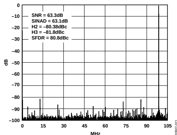
Figure 21. FFT: f_s = 213 MSP, A_{IN} = 100 MHz @ -0.5 dBFS, LVDS Mode
