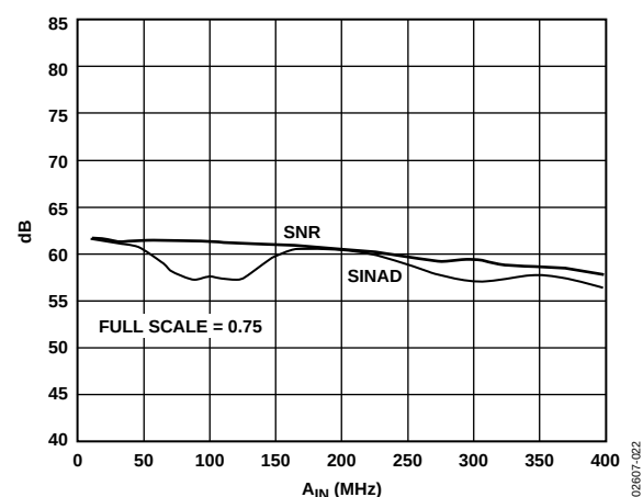
Figure 22. SNR and SINAD vs. A_{IN} Frequency, f_s = 210 MSPS, A_{IN} @ -0.5 dBFS, LVDS Mode, Full Scale = 0.76 V
