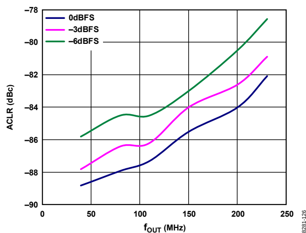
Figure 29. One-Carrier W-CDMA ACLR vs. f_{OUT} over Digital Scale, First Alternate Channel, PLL Off
