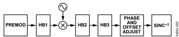
Figure 50. Block Diagram of Digital Datapath
