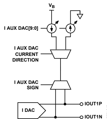
Figure 72. Auxiliary DAC Structure
