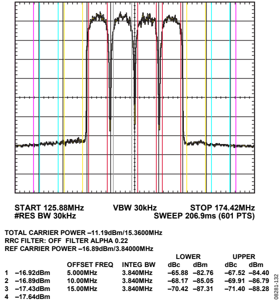
Figure 35. Four-Carrier W-CDMA ACLR Performance, IF = ~150 MHz
