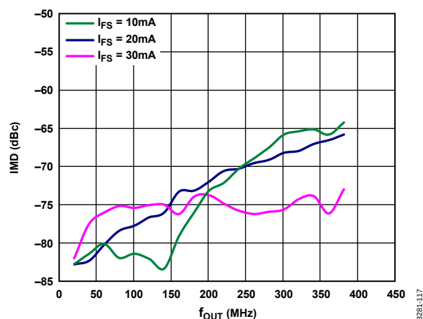
Figure 20. IMD vs. f_{OUT} over I_{FS} , 2× Interpolation, f_{DATA} = 400 MSPS, Digital Scale = 0 dBFS
