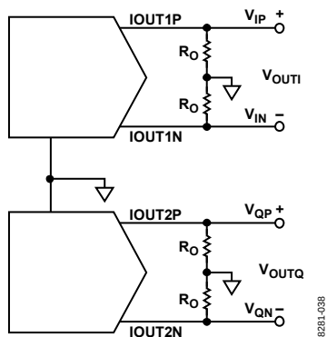
Figure 68. Basic Transmit DAC Output Circuit
