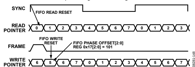
Figure 49. FRAME Input vs. Write Pointer Value, FIFO Rate Mode
