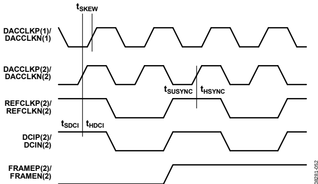
Figure 84. Data Rate Synchronization Signal Timing Requirements, 2× Interpolation
