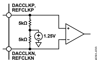
Figure 63. Clock Receiver Input Simplified Equivalent Circuit
