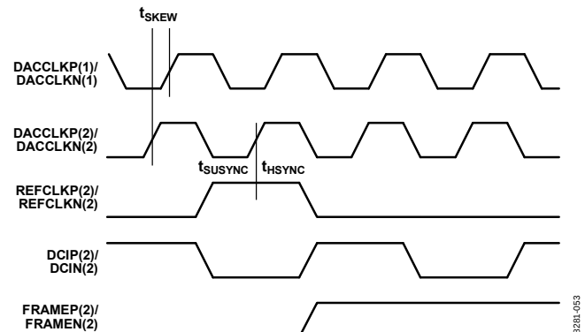
Figure 86. FIFO Rate Synchronization Signal Timing Requirements, 2× Interpolation
