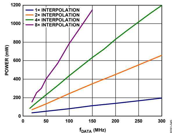
Figure 77. DVDD18 Power Dissipation vs. f_{\text{DATA}} Without Fine NCO or Inverse Sinc
