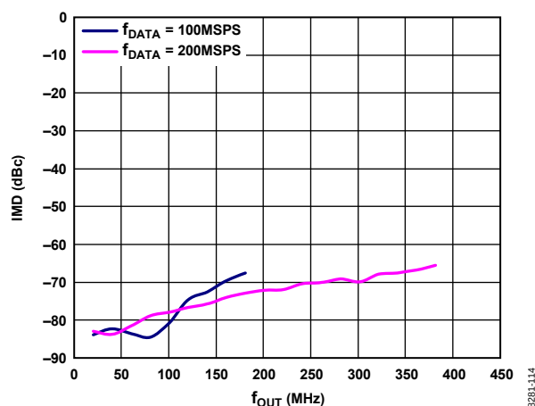
Figure 17. IMD vs. f_{OUT} over f_{DATA} , 4× Interpolation, Digital Scale = 0 dBFS, I_{FS} = 20 mA
