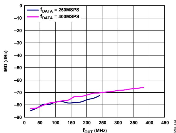
Figure 16. IMD vs. f_{OUT} over f_{DATA} , 2× Interpolation, Digital Scale = 0 dBFS, I_{FS} = 20 mA
