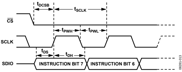
Figure 41. Timing Diagram for Serial Port Register Write
