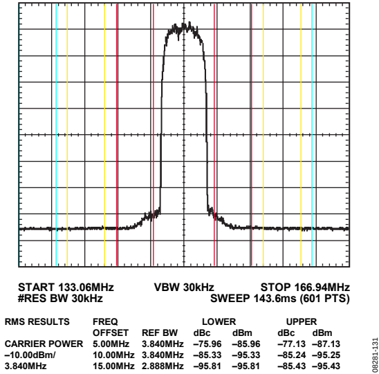
Figure 34. One-Carrier W-CDMA ACLR Performance, IF = ~150 MHz
