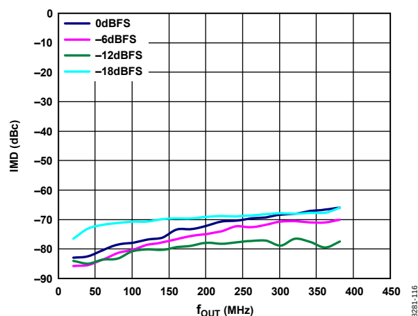
Figure 19. IMD vs. f_{OUT} over Digital Scale, 2× Interpolation, f_{DATA} = 400 MSPS, I_{FS} = 20 mA
