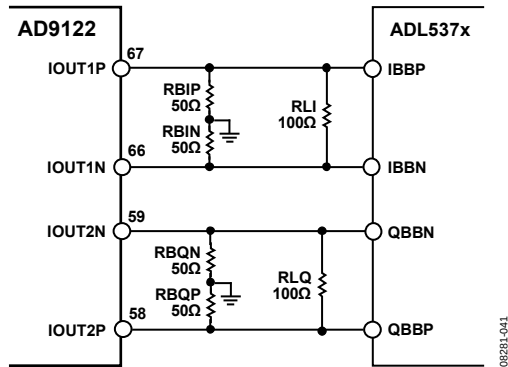
Figure 73. Typical Interface Circuitry Between the AD9122 and the ADL537x Family of Modulators
