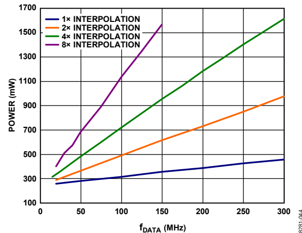
Figure 76. Total Power Dissipation vs. f_{\text{DATA}} Without PLL, Fine NCO, or Inverse Sinc
