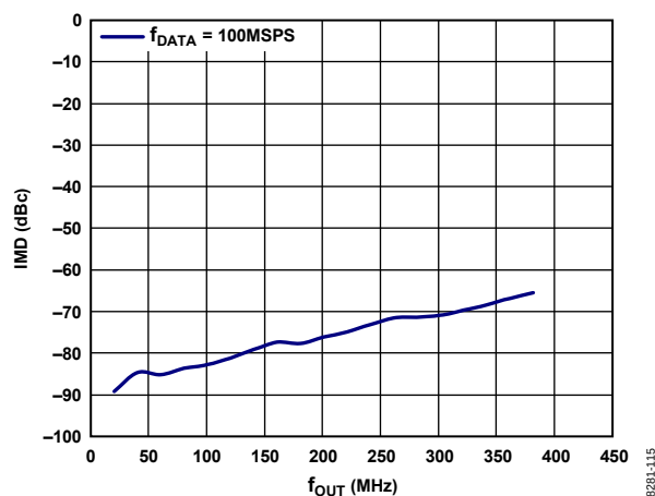
Figure 18. IMD vs. f_{OUT} , 8× Interpolation, f_{DATA} = 100 MSPS, Digital Scale = 0 dBFS, I_{FS} = 20 mA
