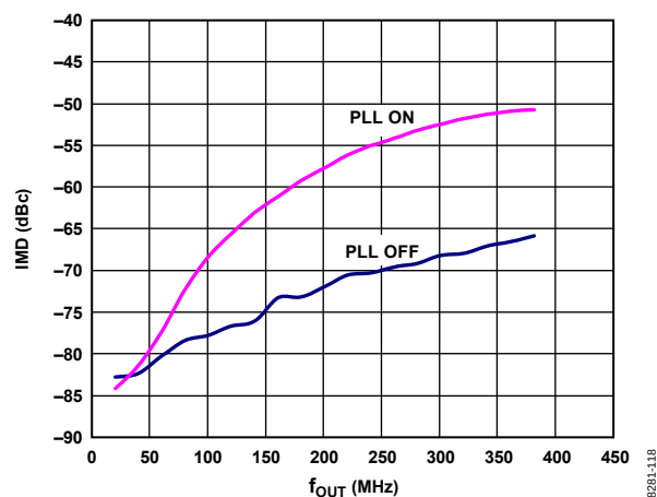
Figure 21. IMD vs. f_{OUT} , 4× Interpolation, f_{DATA} = 200 MSPS, Digital Scale = 0 dBFS, I_{FS} = 20 mA, PLL On and PLL Off
