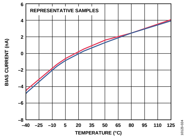
Figure 26. Input Bias Current vs. Temperature
