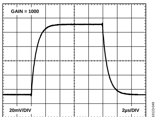
Figure 55. Small Signal Pulse Response ( G = 1000 ), R_L = 600\ \Omega , C_L = 100\ \text{pF}
