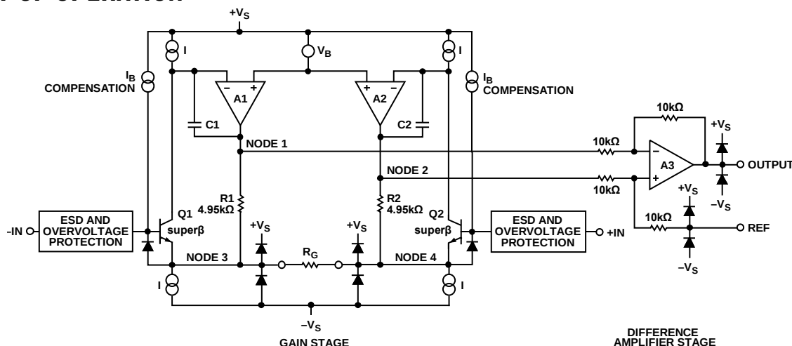
Figure 62. Simplified Schematic
