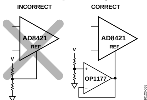
Figure 63. Driving the Reference Pin
