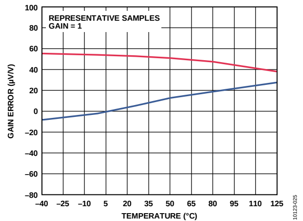
Figure 27. Gain vs. Temperature (G = 1)
