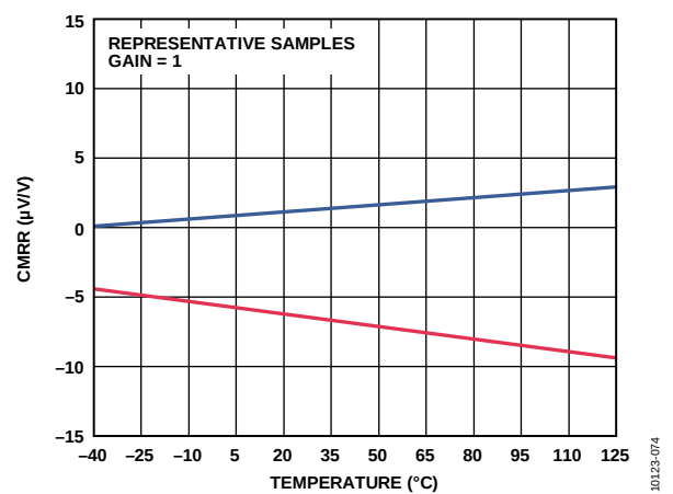
Figure 28. CMRR vs. Temperature (G = 1)
