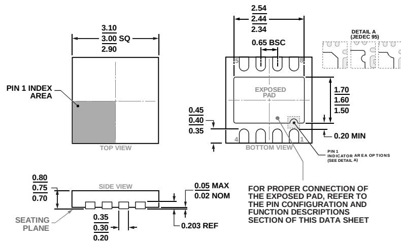
Figure 76. 8-Lead Lead Frame Chip Scale Package [LFCSPP] 3 mm x 3 mm Body and 0.75 mm Package Height (CP-8-19)
