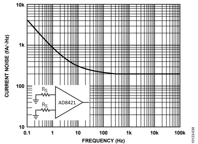
Figure 44. Current Noise Spectral Density vs. Frequency
