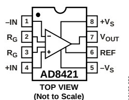
Figure 64. Pin Configuration Diagram
