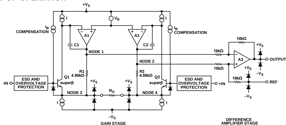
Figure 62. Simplified Schematic
