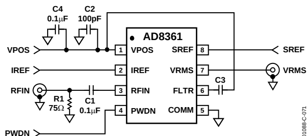
Figure 66. Characterization Board
