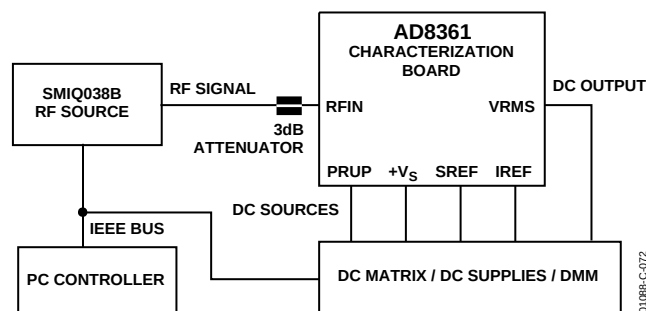
Figure 67. Characterization Setup
