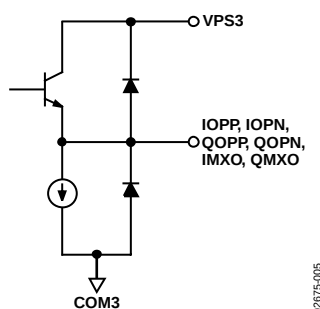
Figure 37. Circuit B
