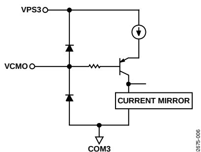
Figure 38. Circuit C
