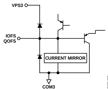
Figure 41. Circuit F
