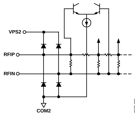
Figure 40. Circuit E
