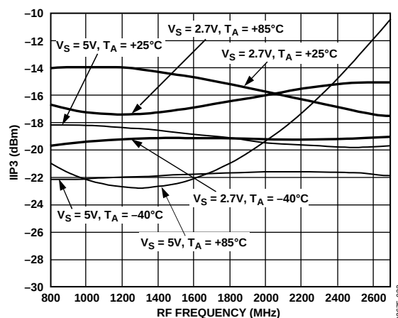
Figure 14. IIP3 vs. F_{LO} , V_{VGIN} = 0.2V , F_{BB} = 1\text{ MHz}
