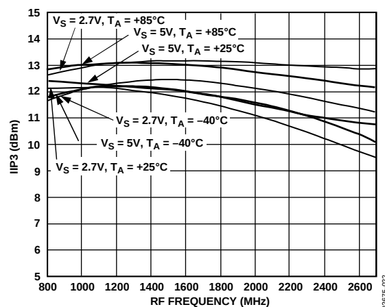
Figure 13. IIP3 vs. F_{LO} , V_{VGIN} = 1.2V , F_{BB} = 1\text{ MHz}
