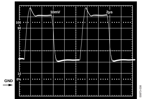
Figure 37. V_S = 5\text{ V} , 0\text{ V} ; Gain-of-2 Inverter Response to 20 mV Step, Centered 20 mV Below Ground
