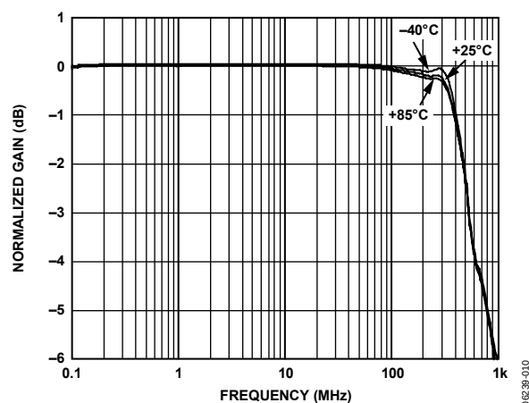
Figure 10. AD8189 Large Signal Bandwidth vs. Temperature, V_{OUT} = 2 \text{ V p-p} , R_L = 150 \Omega
