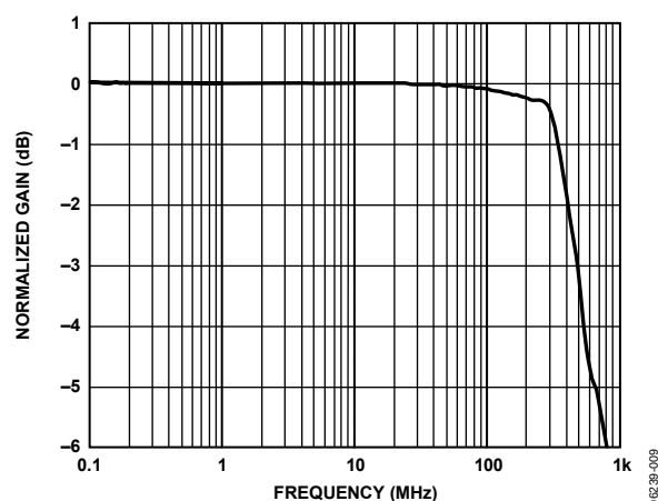
Figure 9. AD8189 Frequency Response, V_{OUT} = 2 \text{ V p-p} , R_L = 150 \Omega
