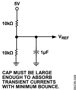
Figure 49. Alternate Method for Synthesis of a False Ground Reference
