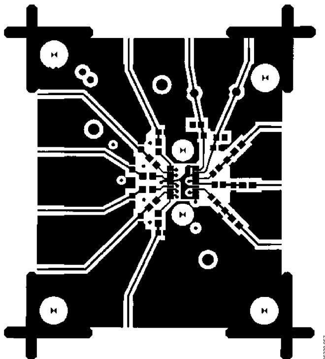
Figure 57. Component Side Board Layout
