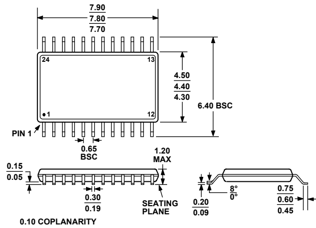
COMPLIANT TO JEDEC STANDARDS MO-153-AD Figure 62. 24-Lead Thin Shrink Small Outline Package [TSSOP] [RU-24] Dimensions shown in millimeters
