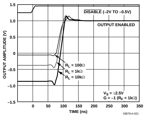
Figure 48. AD8029 \overline{\text{DDISABLE}} Turn-On Timing
