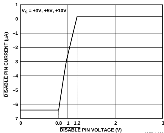
Figure 49. AD8029 \overline{\text{DDISABLE}} Pin Current vs. \overline{\text{DDISABLE}} Pin Voltage
