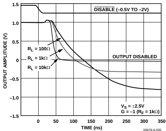
Figure 47. AD8029 \overline{\text{DDISABLE}} Turn-Off Timing
