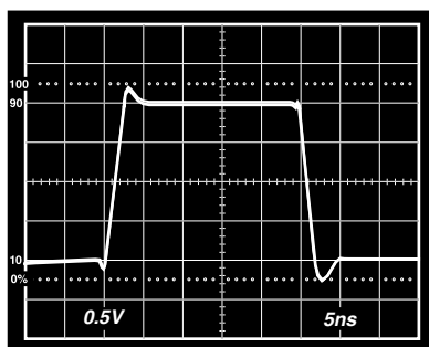
TPC 3. 2 V Step Response, G = +1
