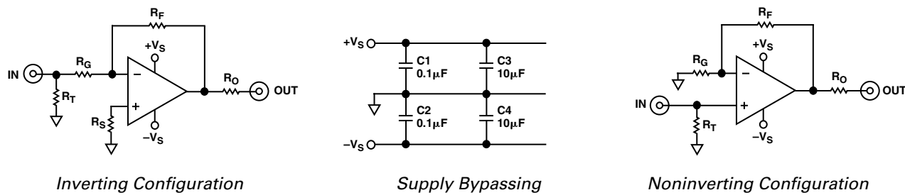
Figure 13. Inverting and Noninverting Configurations for Evaluation Boards
