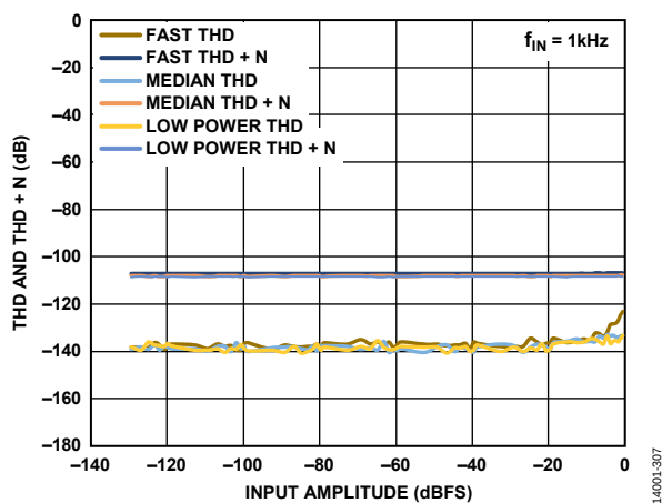
Figure 37. THD and THD + N vs. Input Amplitude, Wideband Filter
