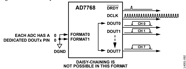
Figure 95. AD7768 FORMATx = 00, Eight Data Output Pins
