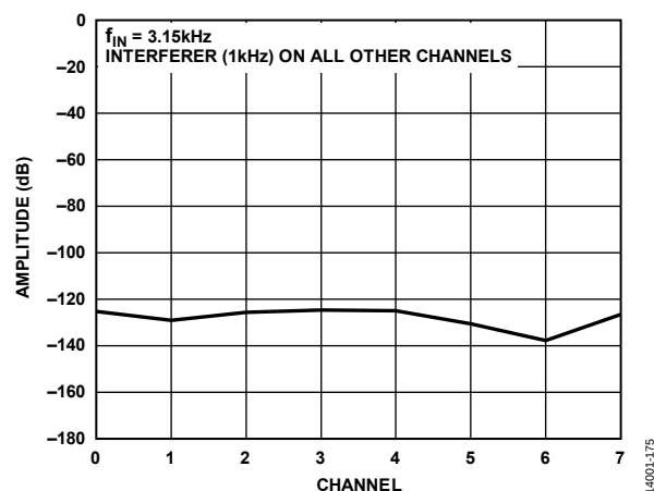
Figure 33. Crosstalk
