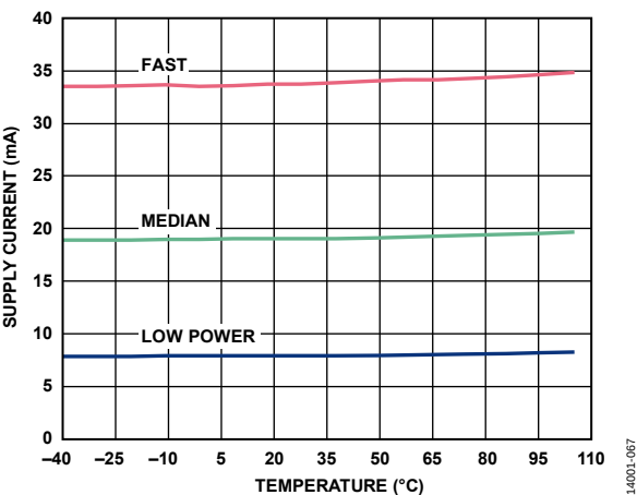
Figure 66. Supply Current vs. Temperature, AVDD2
