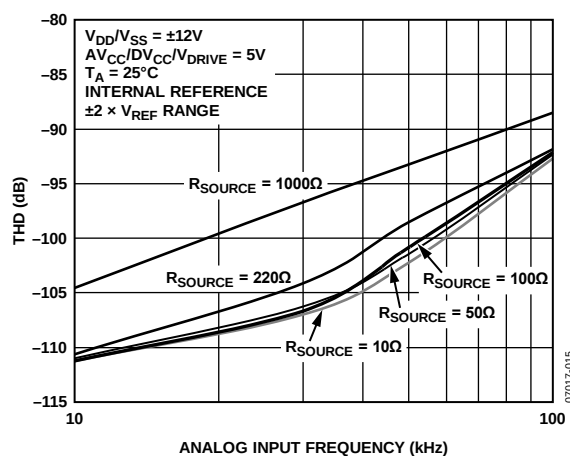
Figure 15. AD7656-1 THD vs. Analog Input Frequency for Various Source Impedances, \pm 2 \times V_{REF} Range
