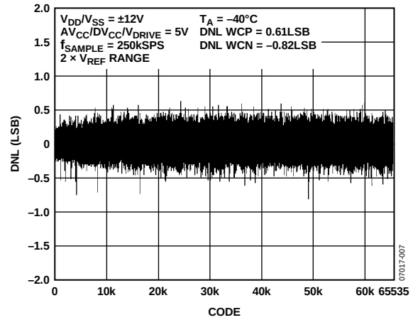
Figure 7. AD7656-1 Typical DNL
