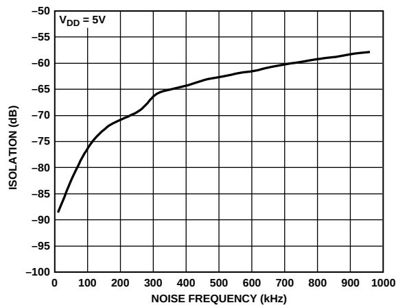
Figure 5. Channel-to-Channel Isolation
