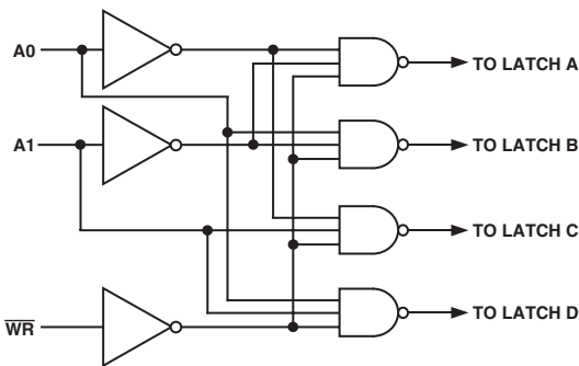
Figure 4. Input Control Logic
