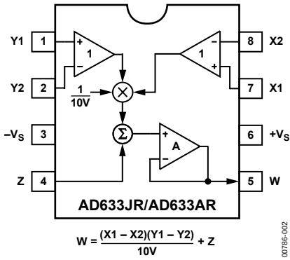
Figure 3. 8-Lead SOIC
