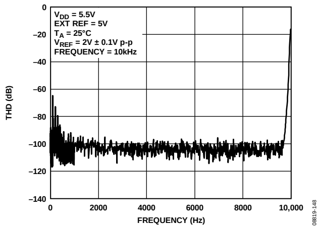
Figure 42. Total Harmonic Distortion
