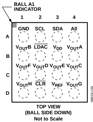
Figure 5. 16-Ball WLCSP
