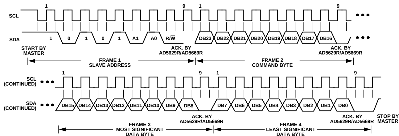
Figure 51. I²C Write Operation
