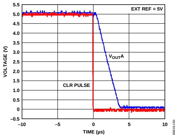
Figure 44. Hardware \overline{\text{CLR}}
