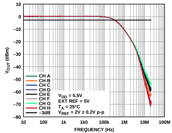
Figure 45. Multiplying Bandwidth
