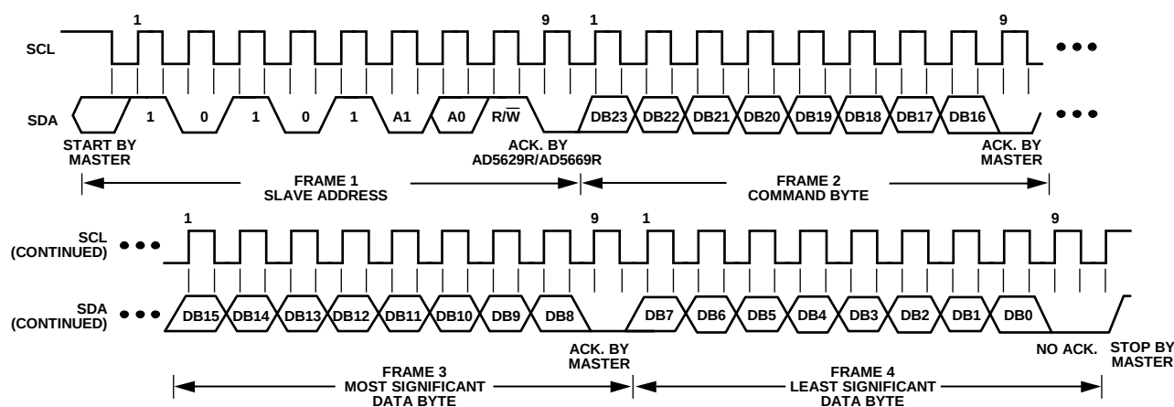
Figure 52. I²C Read Operation
