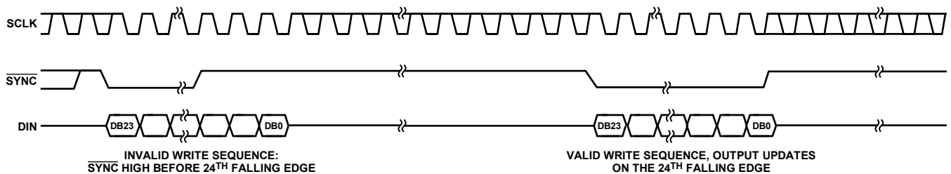
Figure 31. \overline{\text{SYNC}} Interrupt Facility
