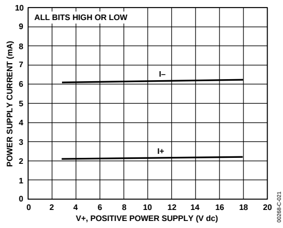
Figure 20. Power Supply vs. V_+
