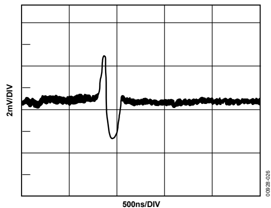
Figure 26. DAC-to-DAC Crosstalk
