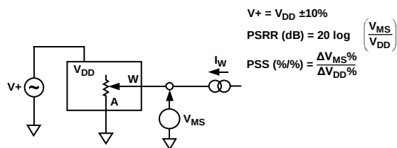
Figure 40. Power Supply Sensitivity (PSS, PSRR)
