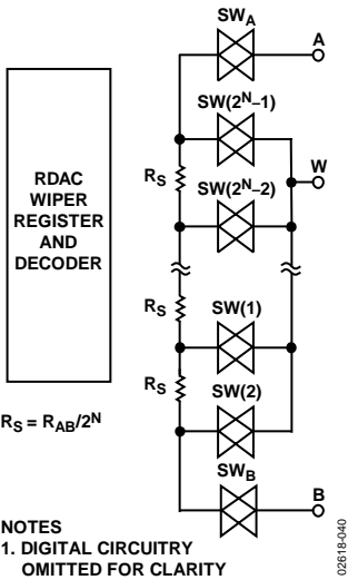
Figure 40. Equivalent RDAC Structure
