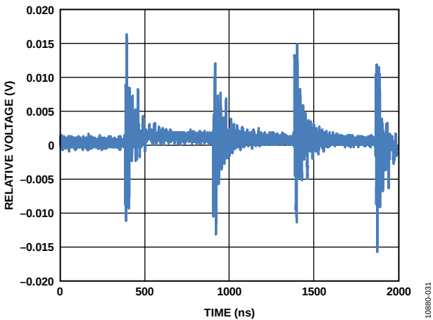
Figure 32. Digital Feedthrough
