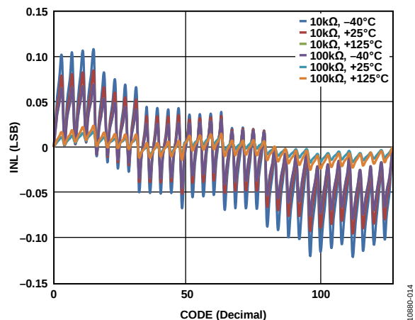
Figure 14. INL vs. Code (AD5122)
