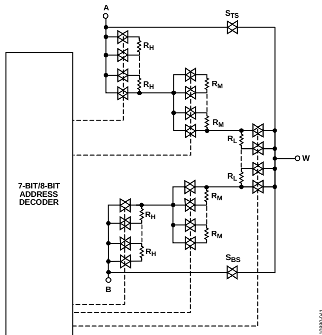
Figure 42. AD5122/AD5142 Simplified RDAC Circuit
