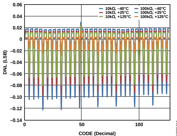
Figure 18. DNL vs. Code (AD5122)
