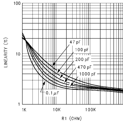
VCO WITHOUT OFFSET
