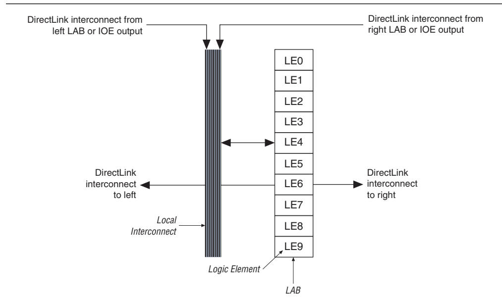
Figure 2-4. DirectLink Connection
