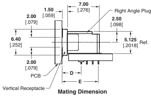
Mating Dimension
