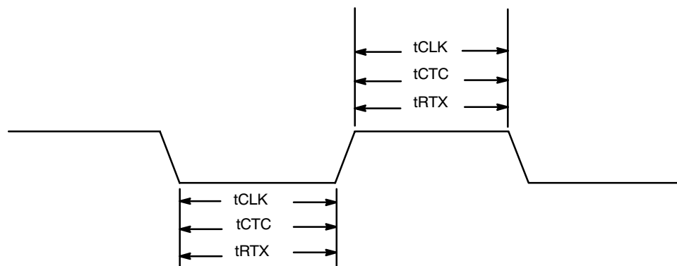
Figure 64. Clock Timing
