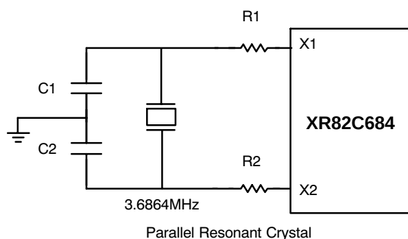
Figure 29. Recommended Schematics for the XTAL Oscillator Circuitry
