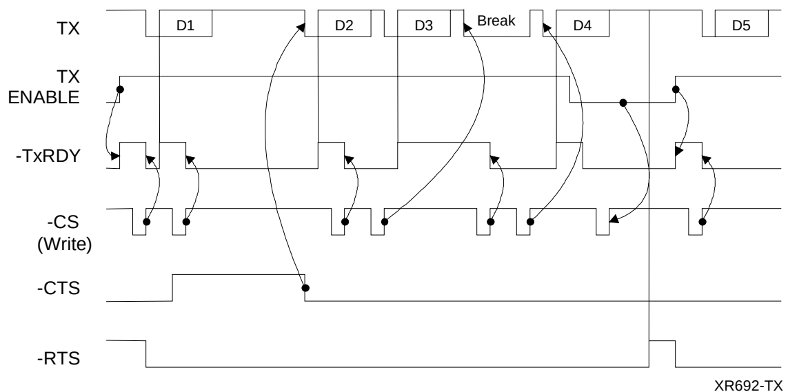
Figure 9: Transmit Timing
