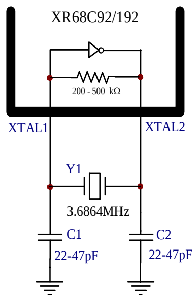
Figure 1: Crystal Connection
