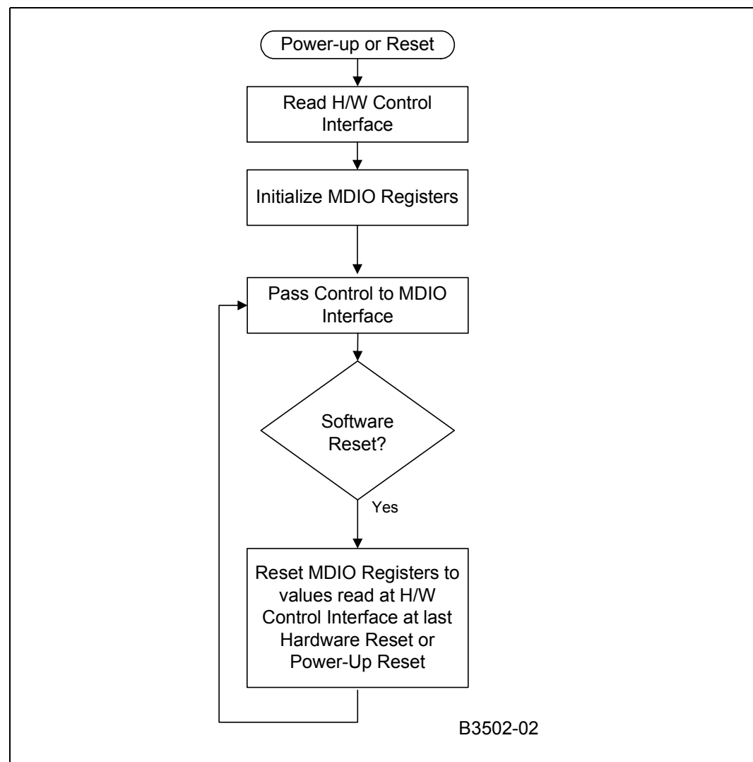
Figure 5 Initialization Sequence
