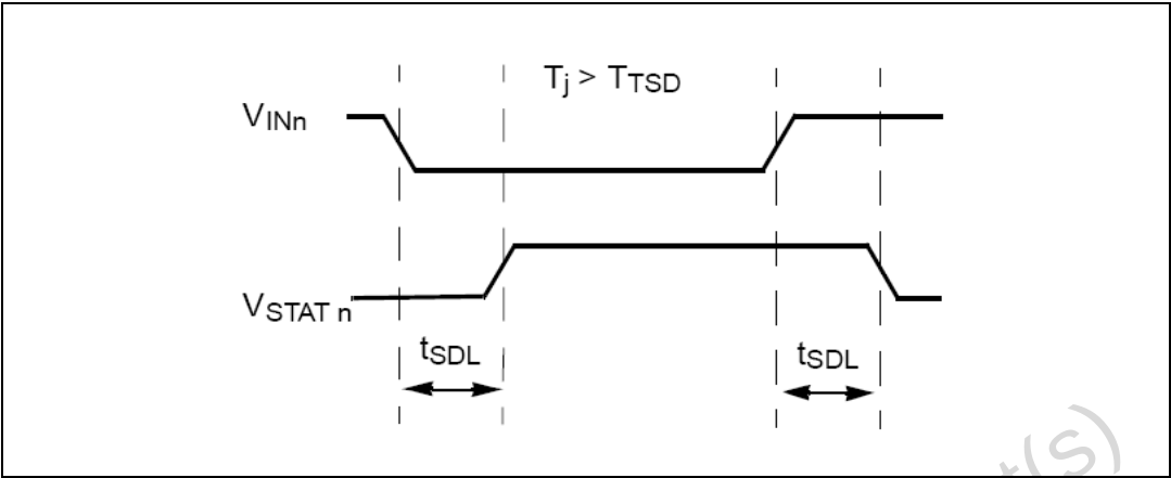
Figure 5. Over temperature status timing
