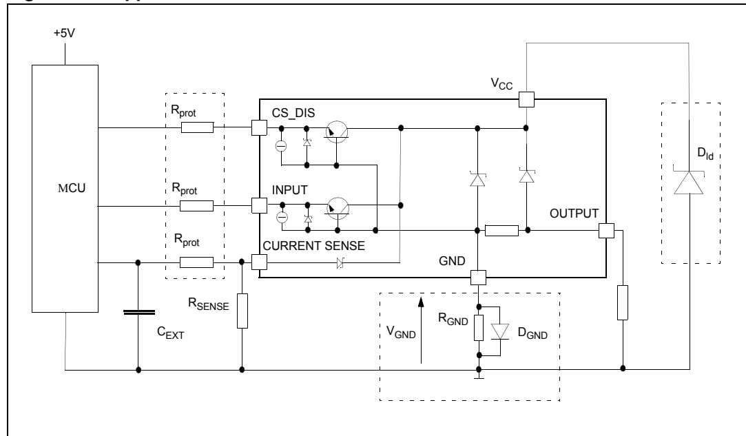
Figure 29. Application schematic (1)
