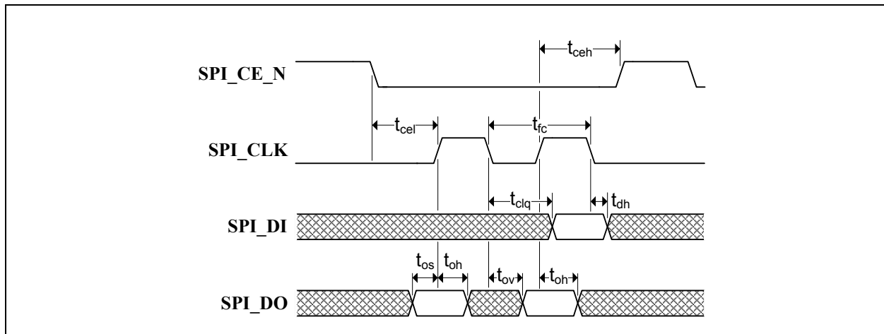
FIGURE 9-5: SPI TIMING
