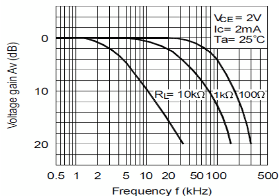
Fig 8 Frequency Response
