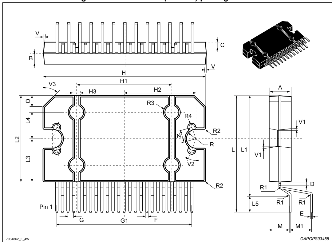
Figure 19. Flexiwatt 25 (vertical) package outline
