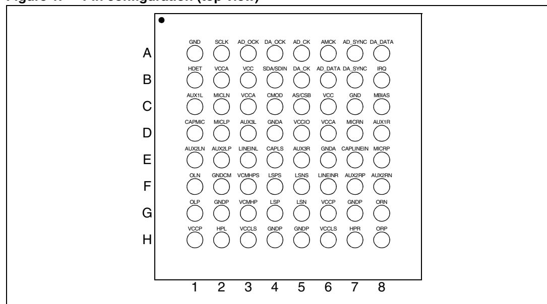
Figure 1. Pin configuration (top view)
