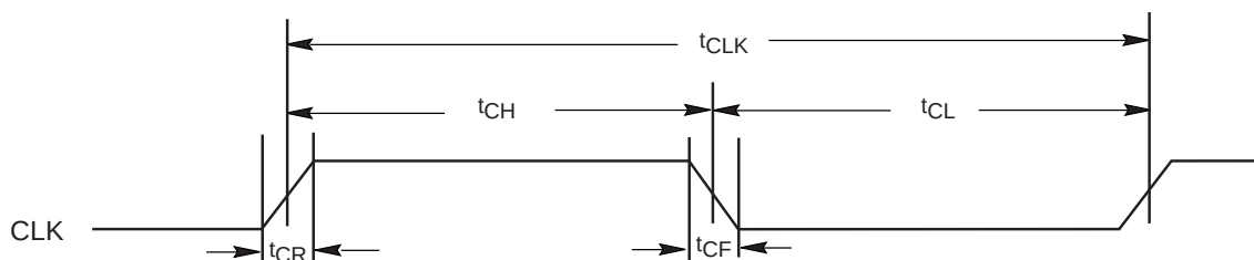
Figure 11.6 CLK Characterization
