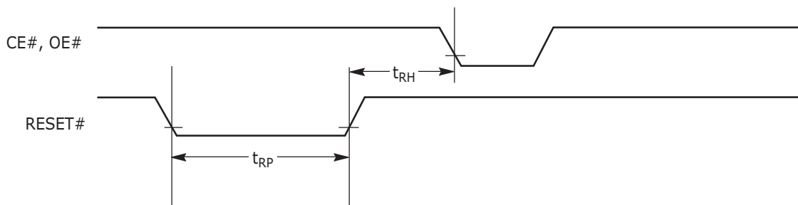
Figure 11.14 Reset Timings
