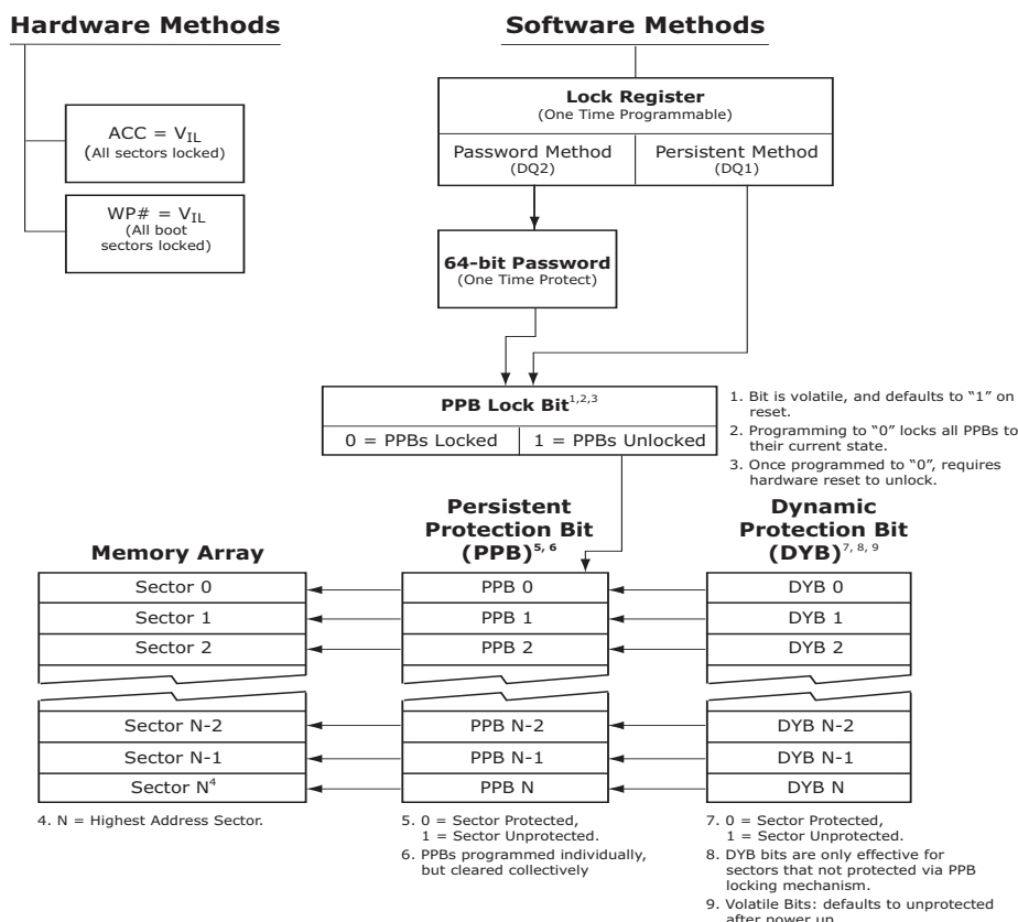
Figure 8.1 Advanced Sector Protection/Unprotection
