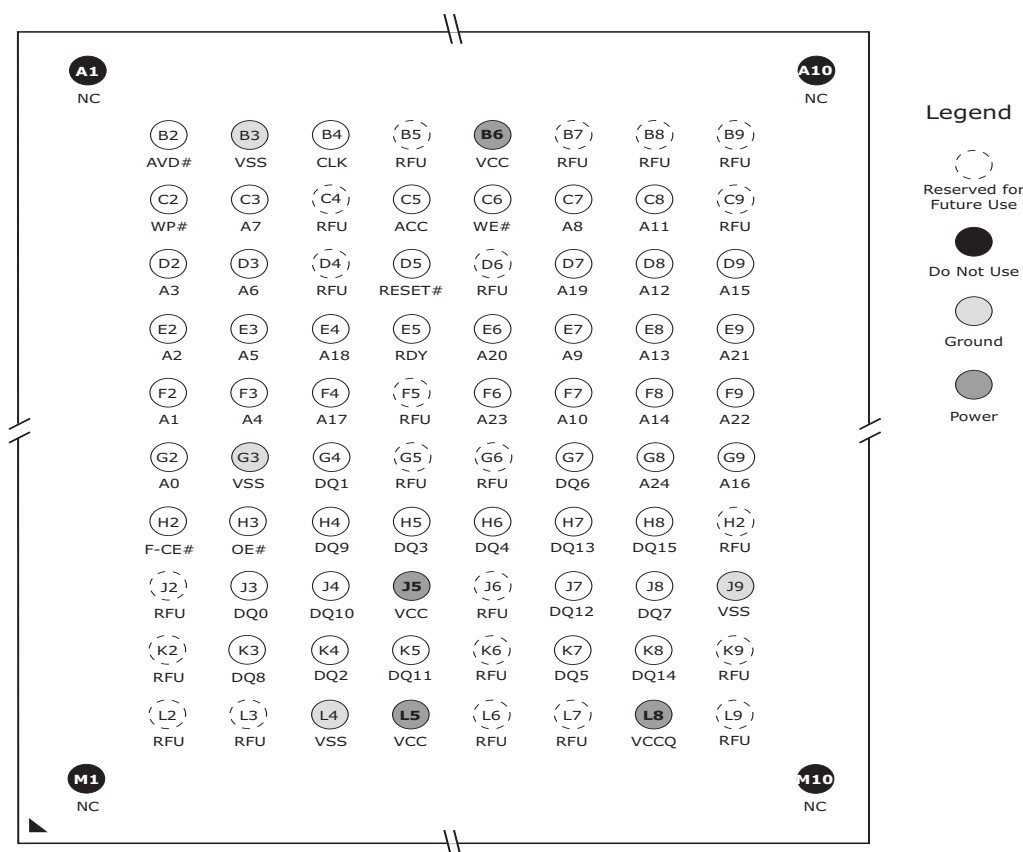
Figure 4.1 84-Ball Fine-Pitch Ball Grid Array, 512, 256 & 128 Mb
