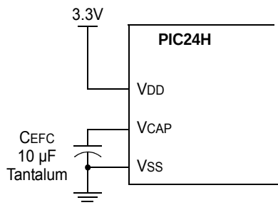
FIGURE 19-1: CONNECTIONS FOR THE ON-CHIP VOLTAGE REGULATOR (1,2,3)
