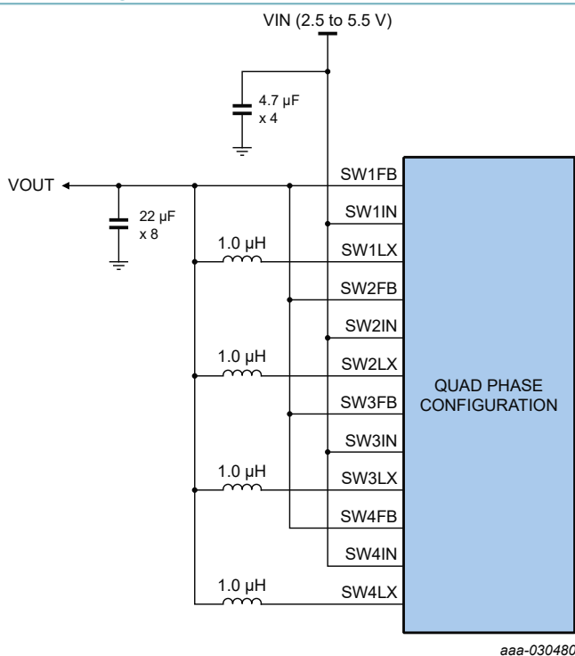
Figure 26. Quad phase configuration
