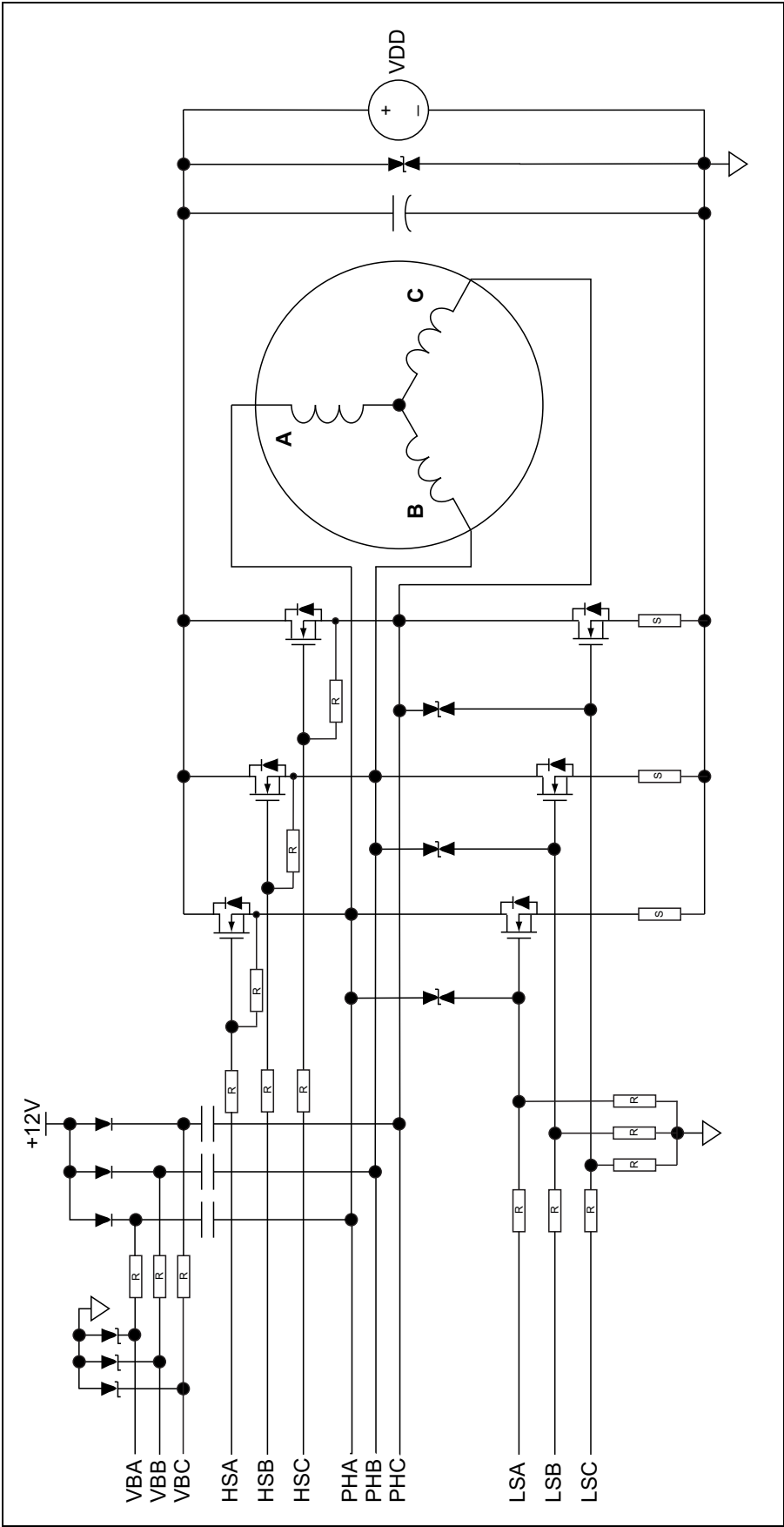
FIGURE 5-3: Overvoltage Protection.
