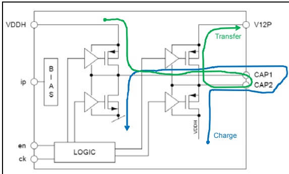
FIGURE 5-1: Charge Pump.
