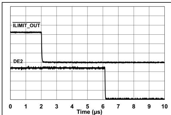
FIGURE 2-3: \overline{\text{ILIMIT\_OUT}} Low to DE2 Message Delay.
