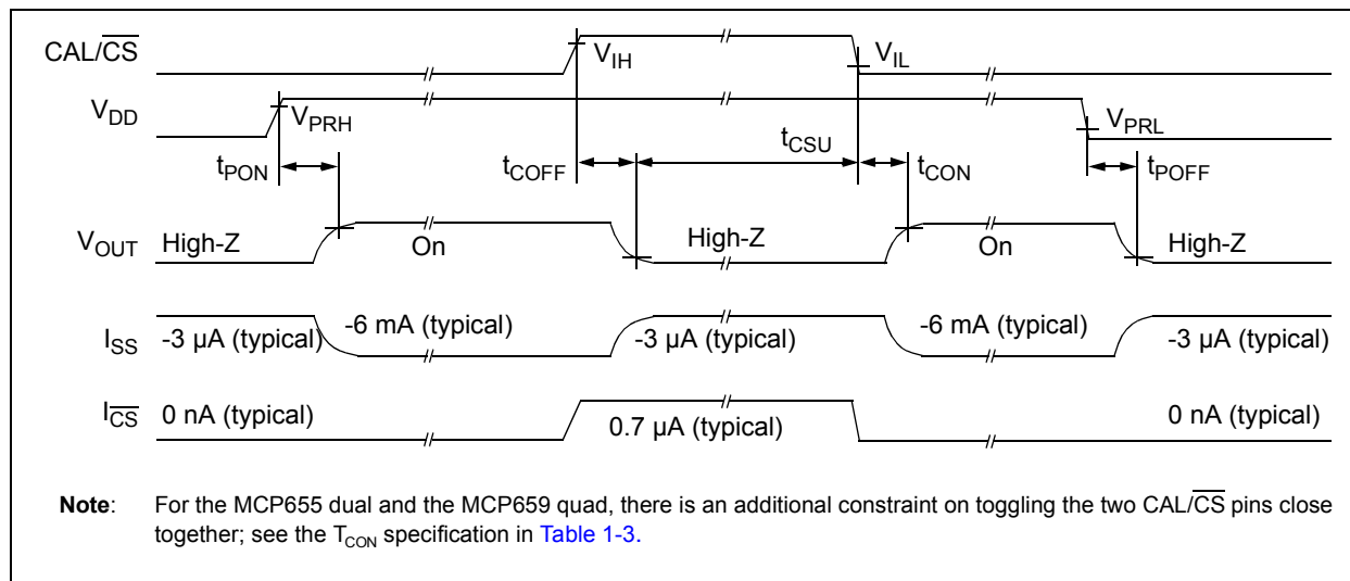
FIGURE 1-1: Timing Diagram.
