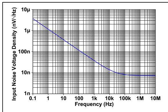
FIGURE 2-32: Input Noise Voltage Density vs. Frequency.
