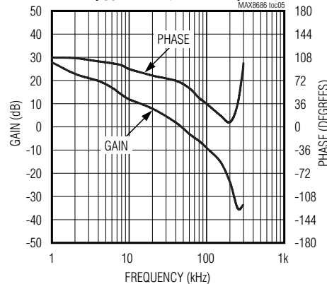
CLOSED-LOOP FREQUENCY RESPONSE ( I_{OUT} = 160A , 8 PHASES)
