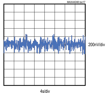
0.1Hz TO 10Hz INPUT VOLTAGE PEAK-PEAK NOISE
